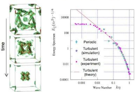
Evolution of vortices Temporally-averaged energy spectrum
